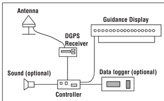
Figure 1. Components of a guidance system.
